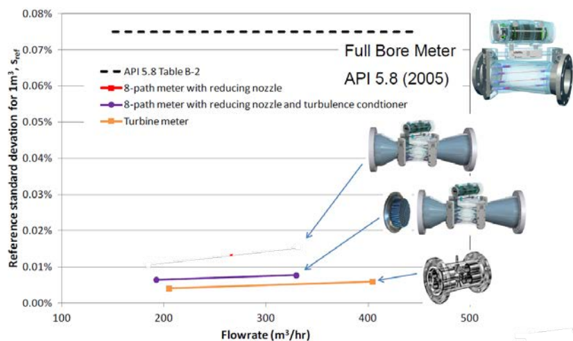
Figure 11: Ultrasonic Meter Sizing
