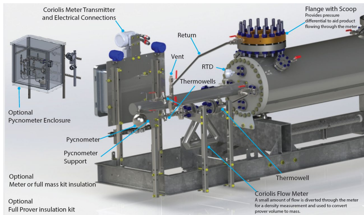
Figure 12: Mass Prover Setup that Includes a Densitometer and Pycnometer
