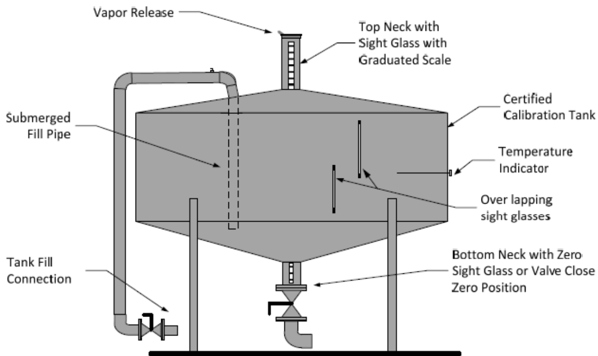
Figure 3: Components of Normal Tank Type Prover
