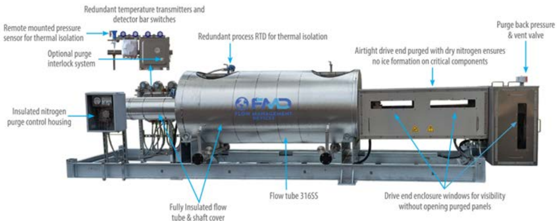
Figure 14: Purge Coverset Details on an SVP
