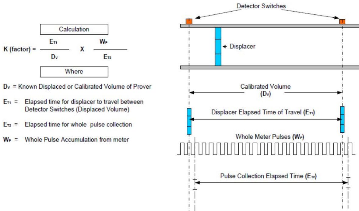
Figure 9: Double Chronometry Pulse Interpolation Formula and Diagram
