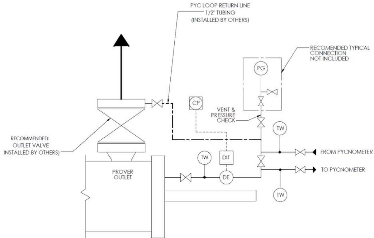
Figure 13: Mass Prover Density P&ID
