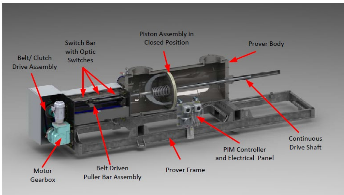
Figure 8: Flow MD SVP Components
