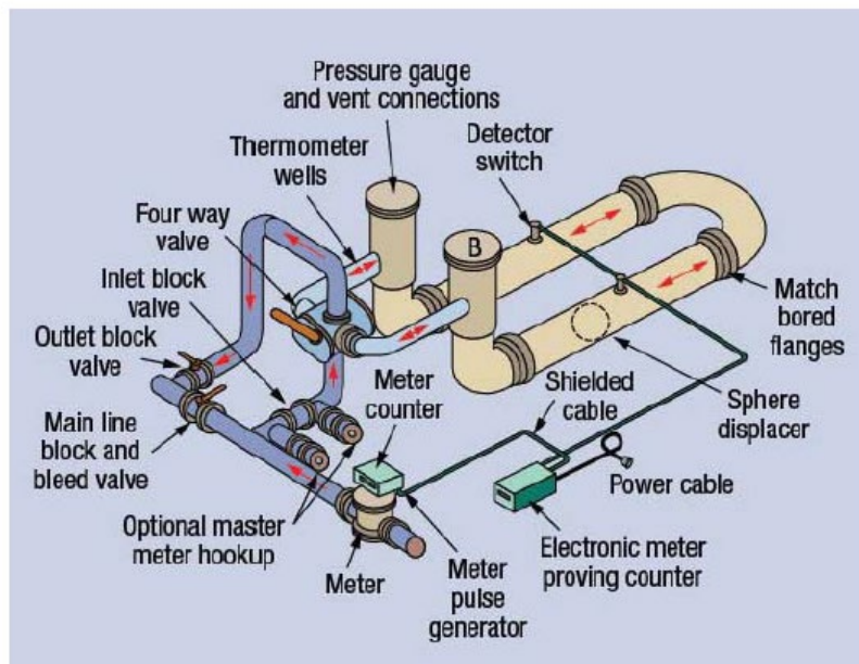
Figure 7: Ball Prover Components
