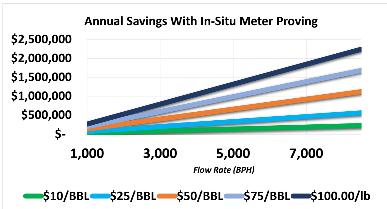
Figure 1: Difference in Potential Losses Of 0.02% Accuracy Versus 0.05% (Proving Versus Not Proving)
